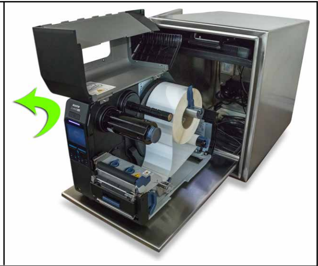
Printer door opens allowing easy label stock replacement.
