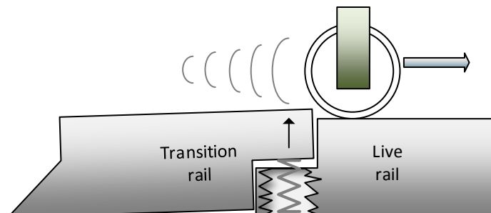
Once the trolley is completely on the live rail, the transition rail rises off the live rail so it will not affect weighments.
