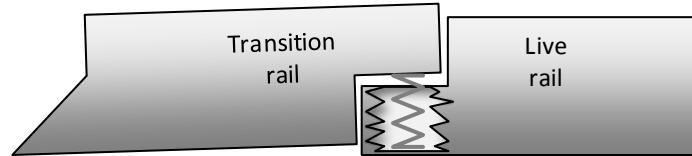
The transition rail in an unloaded state.
