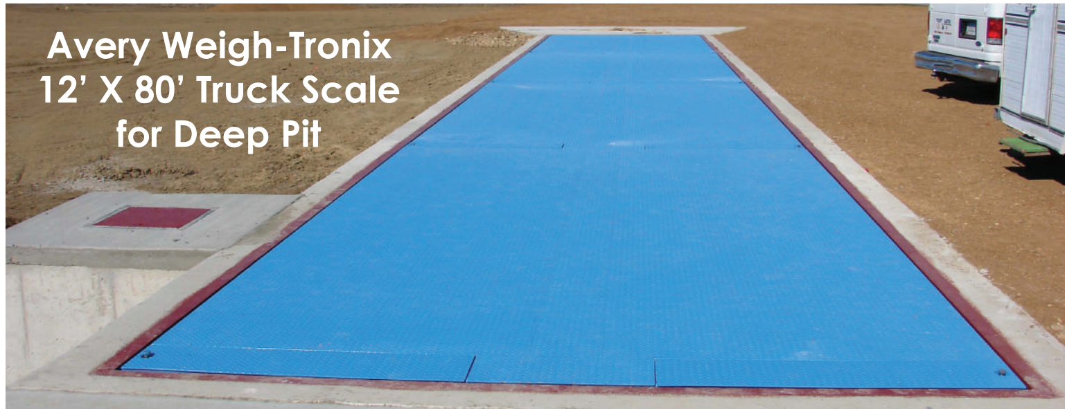
The completed scale features a flush ground installation with a long-lasting metal deck.
