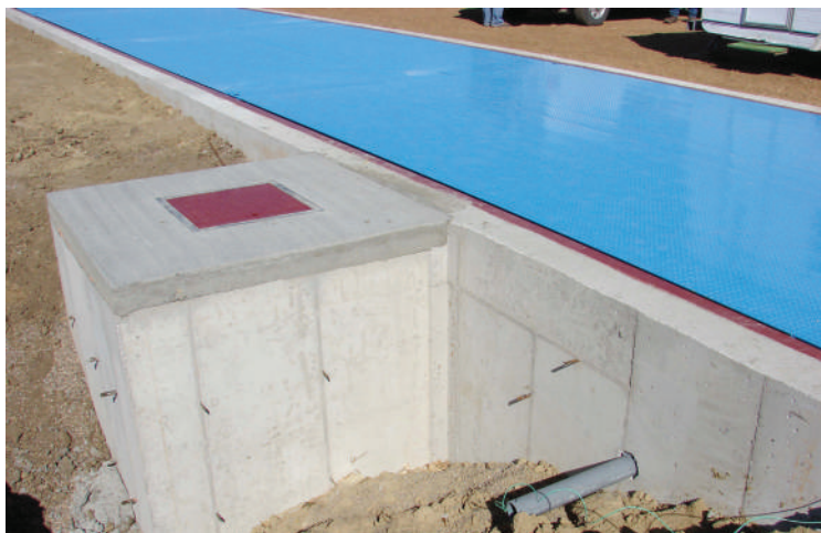
Neck access to enter scale pit with combination sump pit
